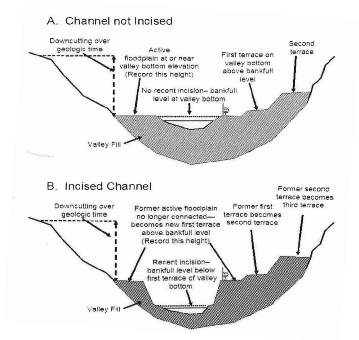
Figure 5-12. Relationship between bankfull channel and incision
