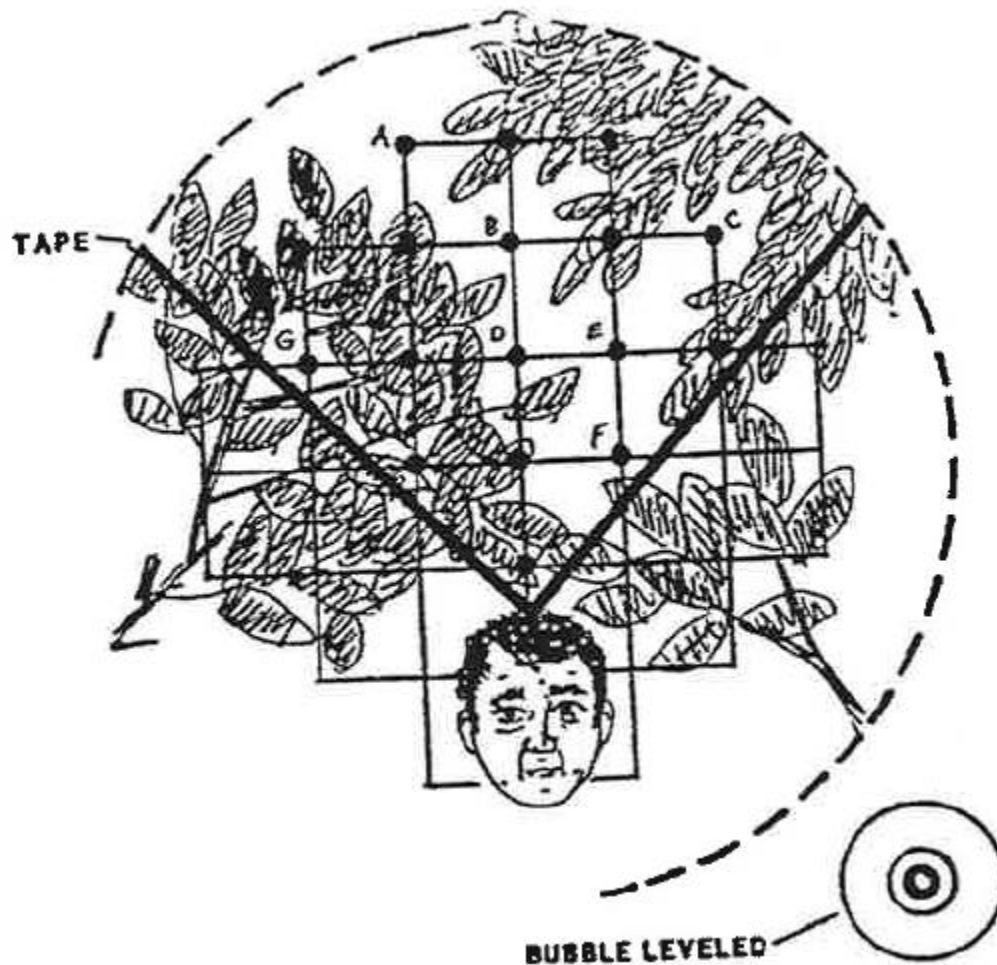
Figure 5-14. Schematic of modified convex spherical densiometer
