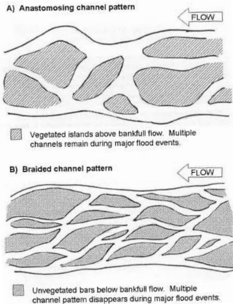
Figure 5-20. Types of multiple channel patterns
